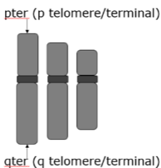
submetacentric
